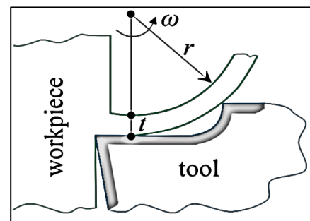
Figure 5. Formation of chip curl-up radius
